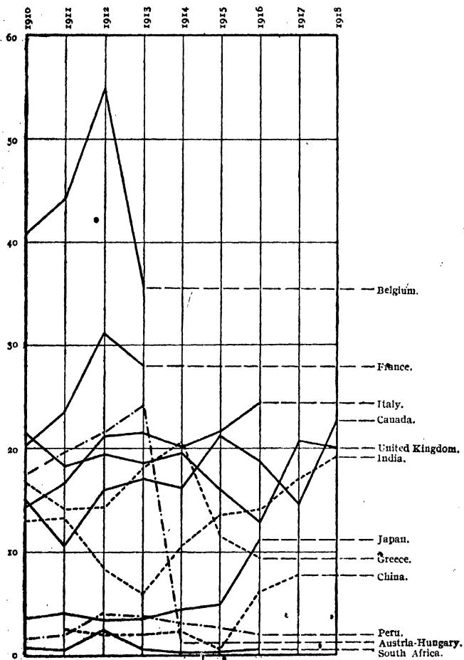
DIAGRAM II.—SHOWING ANNUAL PRODUCTIONS OF LEAD OF THE SMALLER PRODUCING COUNTRIES (THOUSANDS OF METRIC TONS)
